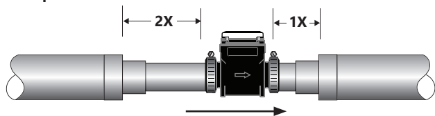
Reduced Pipe
