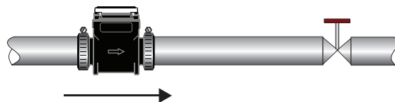
Better Installation
