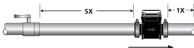
Swirling Flow: Partially Open Butterfly Valve
