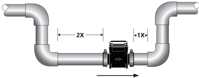
Elbows
