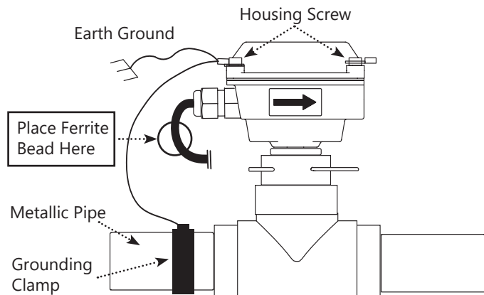
Grounding Diagram
